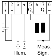
Type -H1, -H2, -H3
